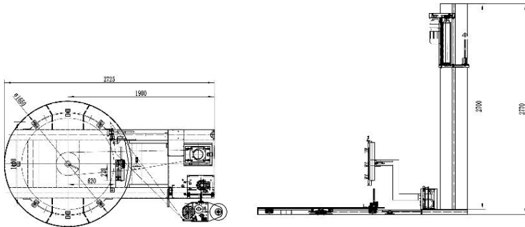
LAYOUT SIZE DRAWING (MM)
