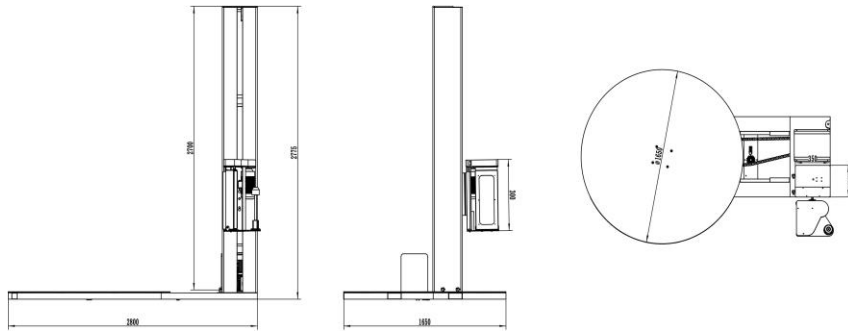
LAYOUT SIZE DRAWING (MM)
