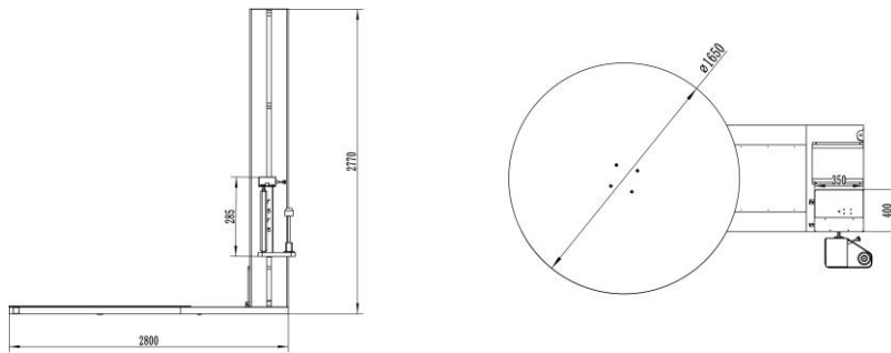
LAYOUT SIZE DRAWING (MM)
