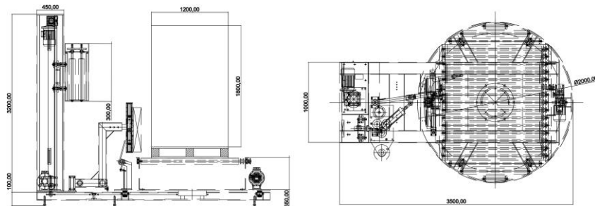
LAYOUT SIZE DRAWING (MM)
