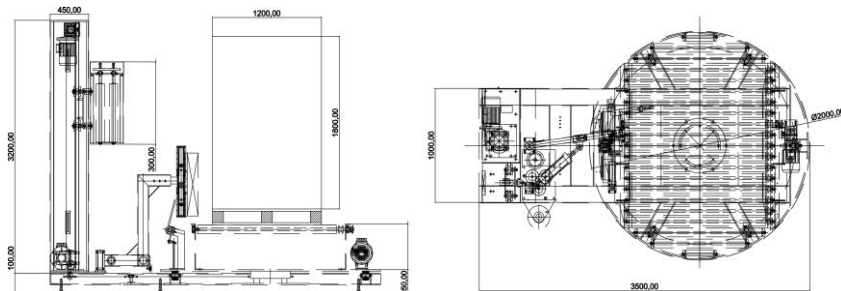
LAYOUT SIZE DRAWING (MM)
