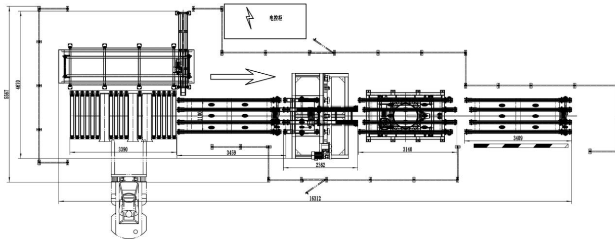
LAYOUT SIZE DRAWING (MM)
