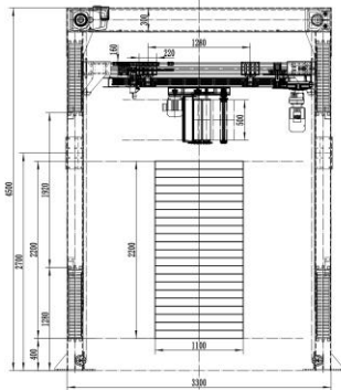
LAYOUT SIZE DRAWING (MM)
