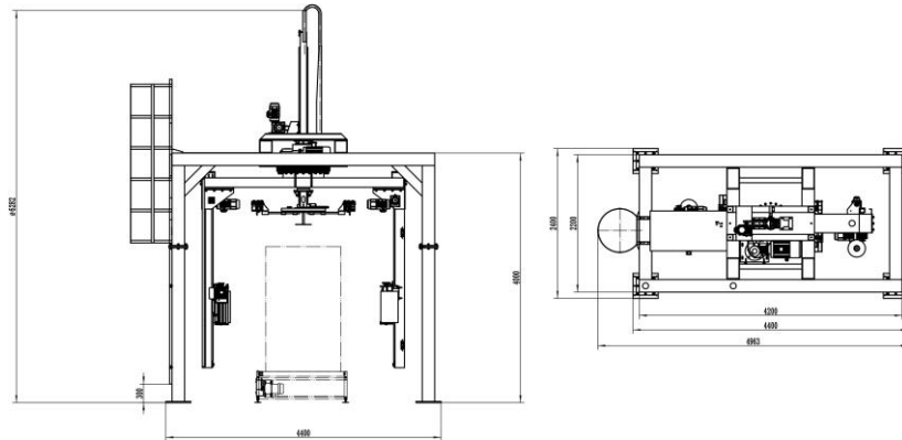
LAYOUT SIZE DRAWING (MM)
