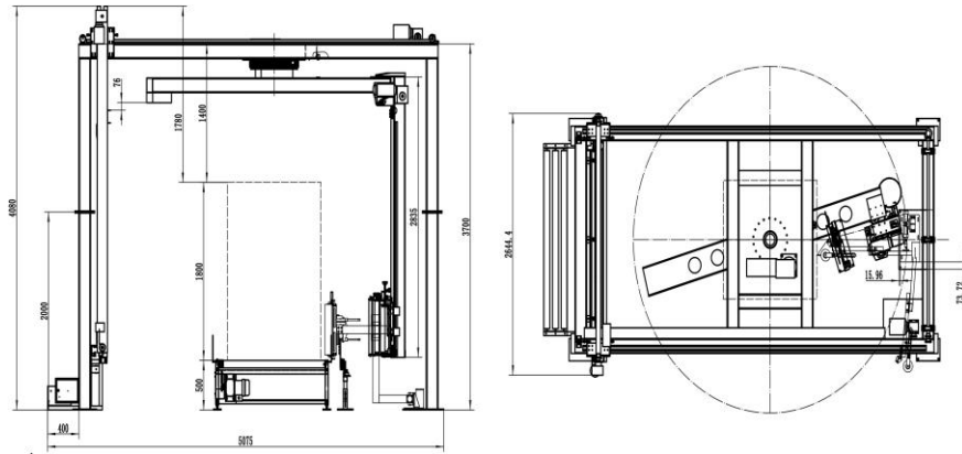
LAYOUT SIZE DRAWING (MM)
